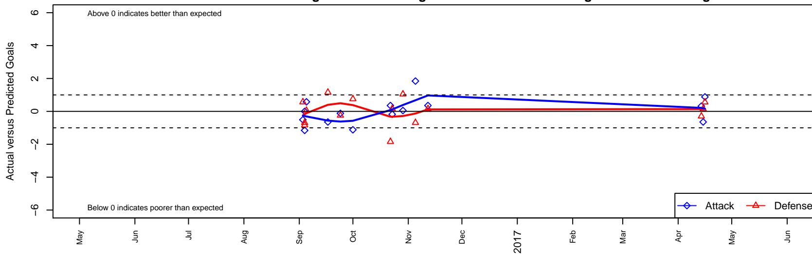
Surrey United B02 Dots are actual minus expected GF (blue circles) and GA (red triangles). Blue line is smoothed change in attack strength. Red is smoothed change in defense strength.
